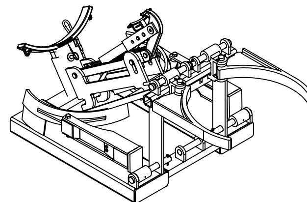
TOP LIP POLY DRUM LIFTER -CAPACITY: 1,100 LBS. -OVERALL DIMENSIONS: 30 1/8" H x 29" W x 48 7/16" L
