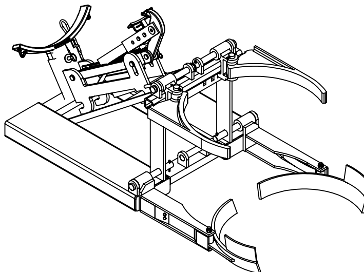
BOTTOM LIP POLY DRUM LIFTER -CAPACITY: 800 LBS. -OVERALL DIMENSIONS: 30 1/8" H x 29" W x 56 7/16" L
