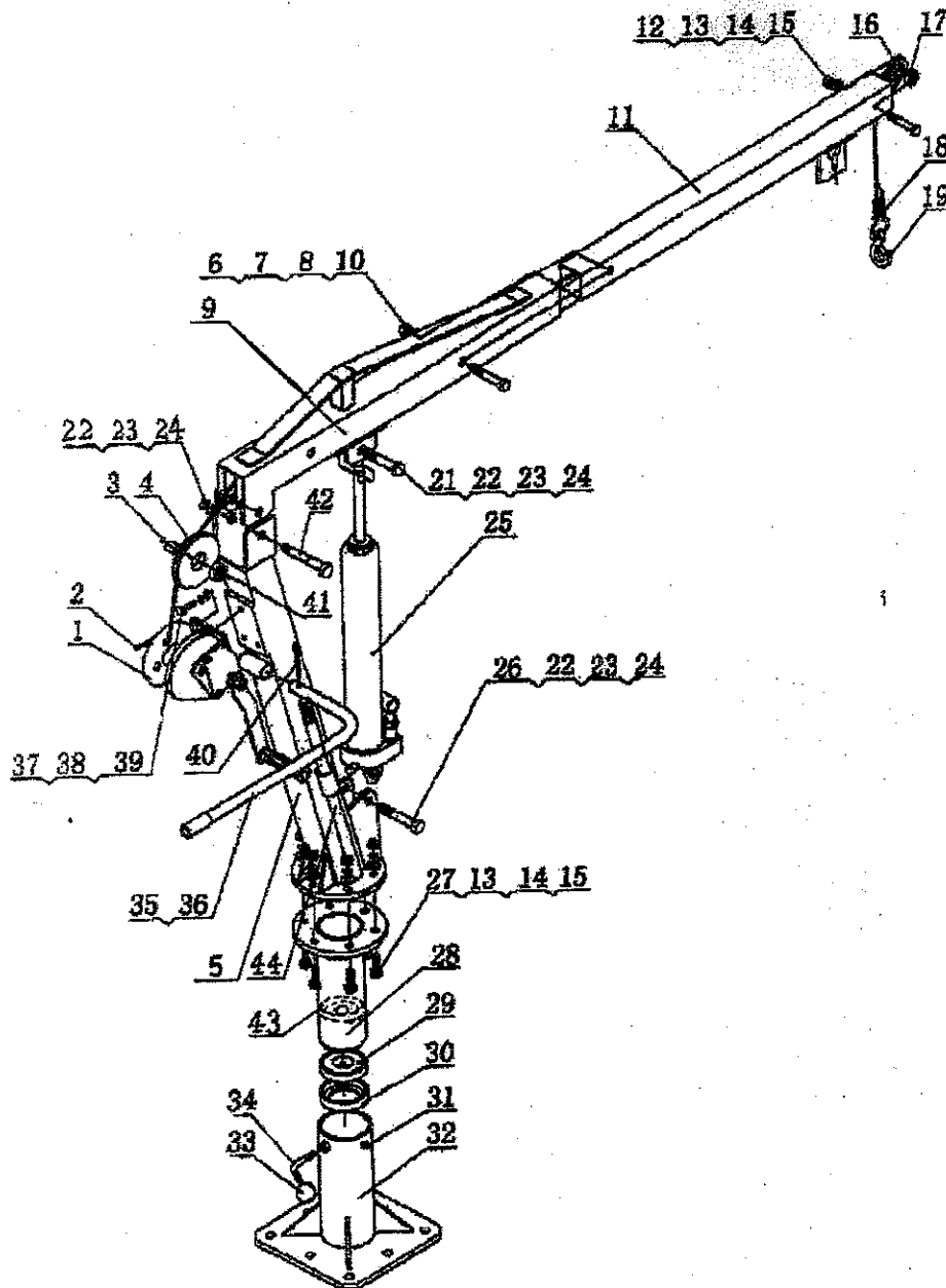
Parts Diagram
