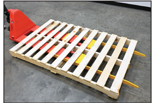
7¼"W x 2"H USABLE FORK POCKETS
