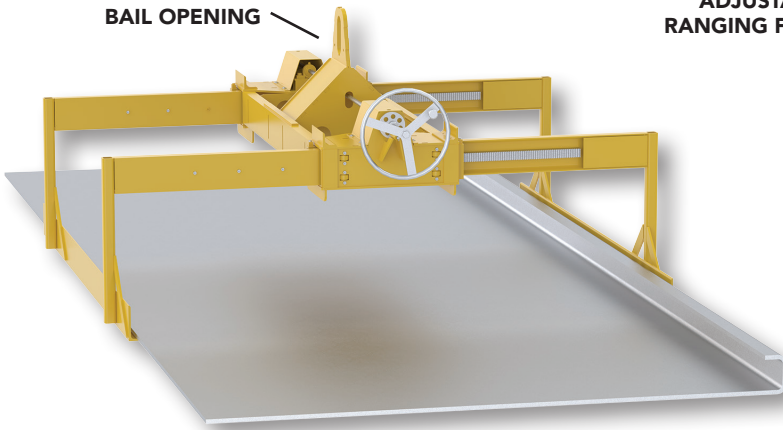
3"W x 7"H BAIL OPENING
